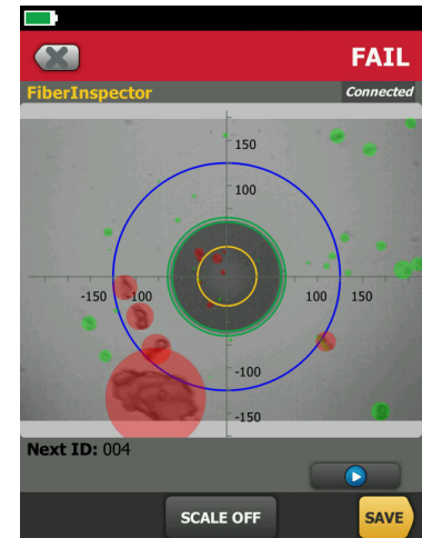
FiberInspector probe
