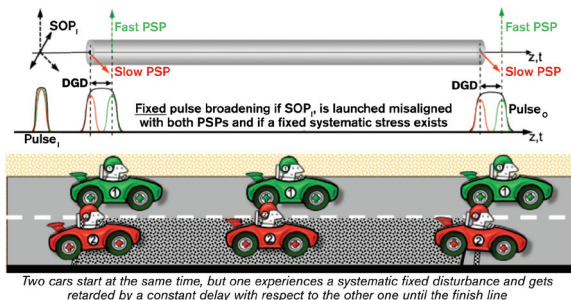
Figure 17 – Pulse Whose SOP is Aligned with Both PSPs Experiences Fixed DGD and Pulse Broadening
