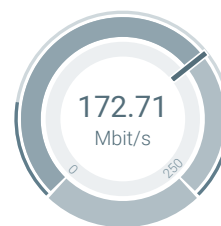
Upload ✓
