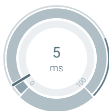
Latency ✓
