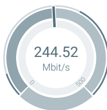
Download ✓
