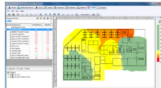
AirMagnet Survey
