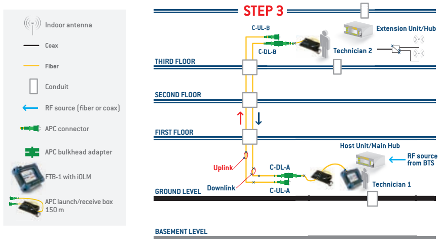
Figure 41 – Two technicians: Preparation for DL fiber test
