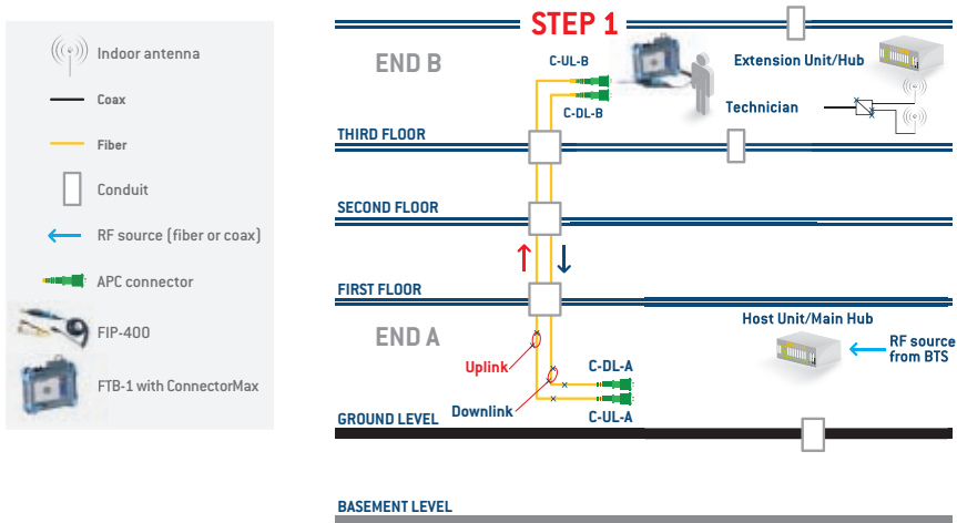
Figure 34 – One technician: End B connector inspection
