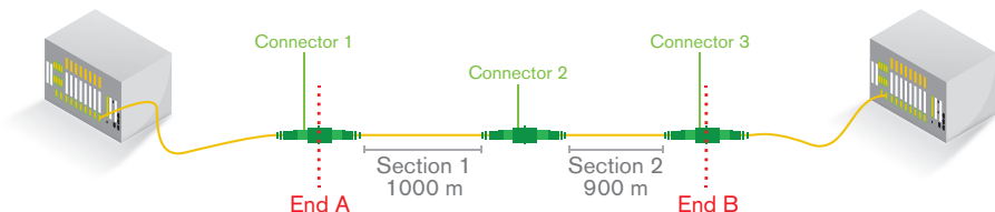
Figure 6 – Typical DAS fiber installation
