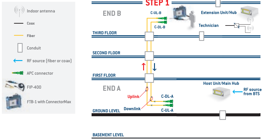
Figure 25 – One technician: End B connector inspection
