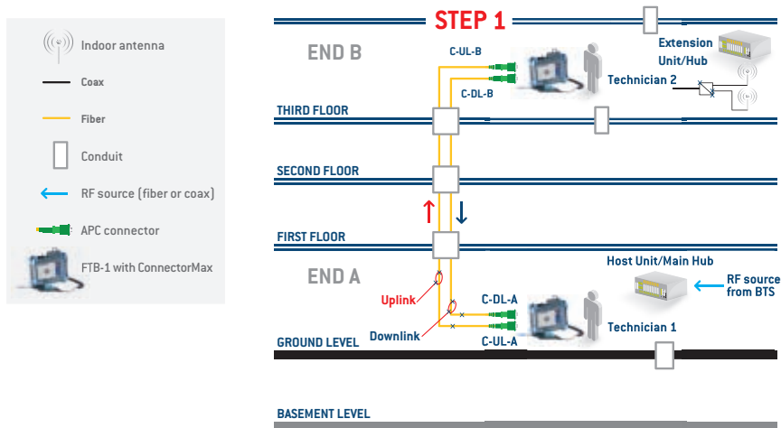
Figure 30 – Two technicians: End A and B connector inspection
