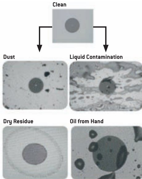
Figure 20 – Clean connector endface vs. different contaminant types
