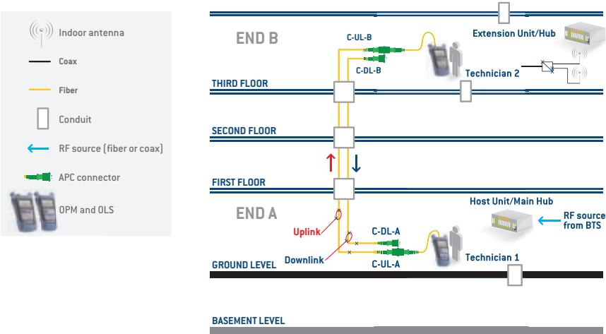
Figure 43 – Loss testing using an OPM and OLS
