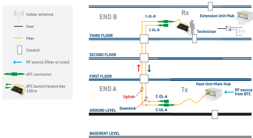
Figure 49 – Connecting the receive fiber at the Rx
