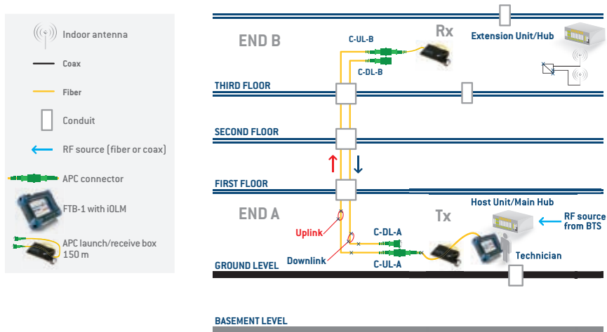
Figure 50 – Performing the iOLM (OTDR) test from the Tx
