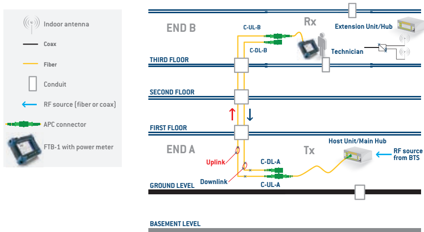
Figure 48 – Power measurement at the Rx location
