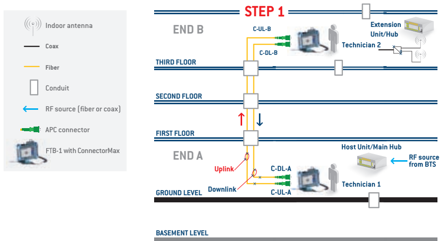
Figure 39 – Two technicians: End A and B connector inspection
